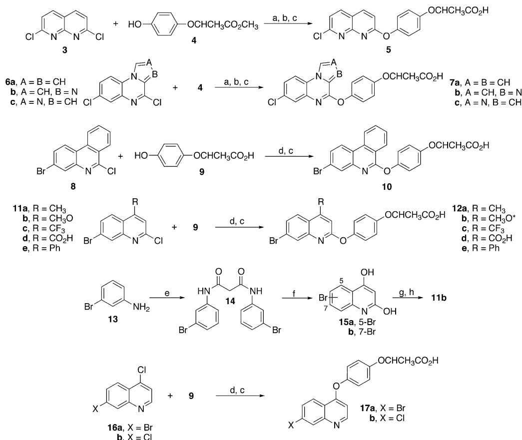
Scheme 1. Reagents: (a) K 2 CO 3 /CH 3 CN (method A); (b) aq NaOH/THF; (c) aq HCl; (d) K 2 CO 3 /DMF (method B); (e) diethyl malonate; (f) Eaton's reagent; (g) Me 2 SO 4 , K 2 CO 3 /acetone; (h) POCl 3 . *Via method A.
